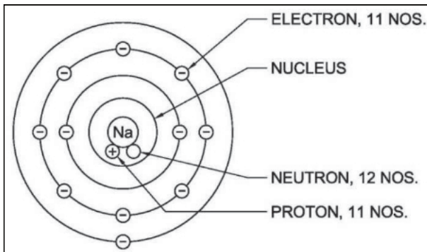
Figure 3.4: Atomic structure of sodium atom. Image by Rajan (2021) via https://www.researchgate.net/figure/Atomic-structure-of-sodium-atom_fig1_349498027 (copyright-free).
